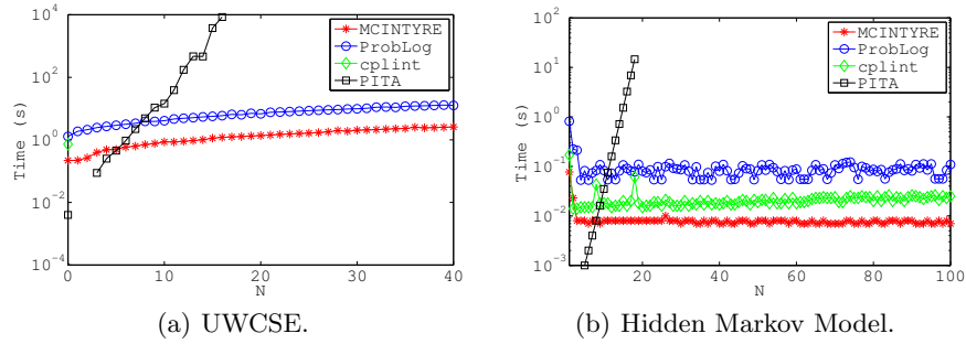
Fig. 5. UWCSE and Hidden Markov Model
